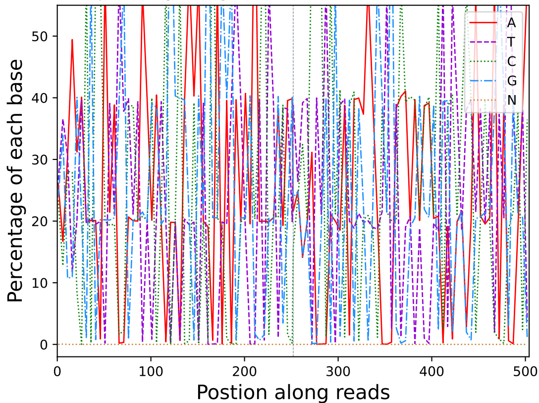
Base percentage along reads (R10102)
